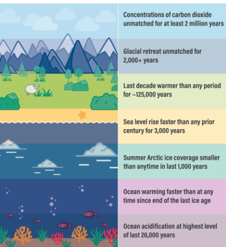
Source: IPCC AR6. WORLD RESOURCES INSTITUTE
